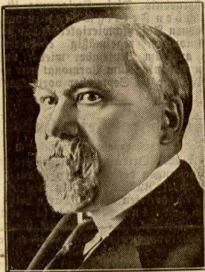
Poincaré †.
